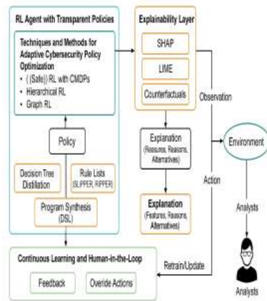
Fig1. Architecture Diagram
